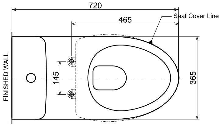
PLAN / TOP ELEVATION
