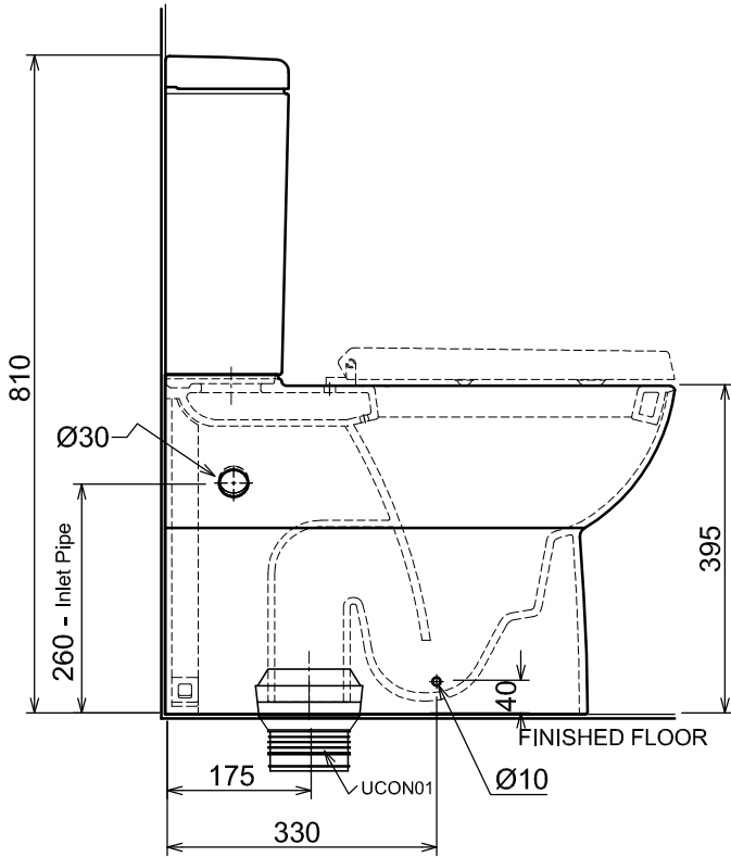
SIDE ELEVATION
