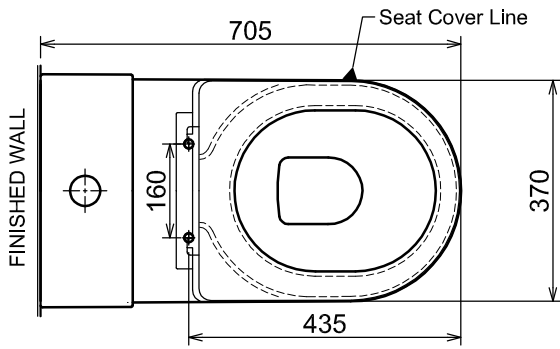
PLAN / TOP ELEVATION
