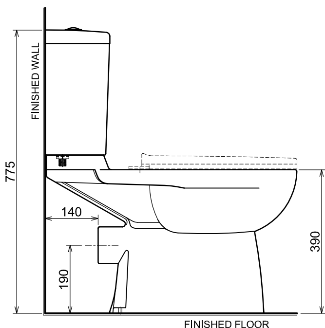
SIDE ELEVATION
