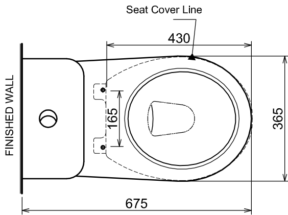
PLAN / TOP ELEVATION
