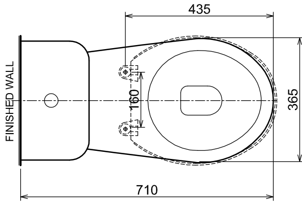
PLAN/TOP ELEVATION
