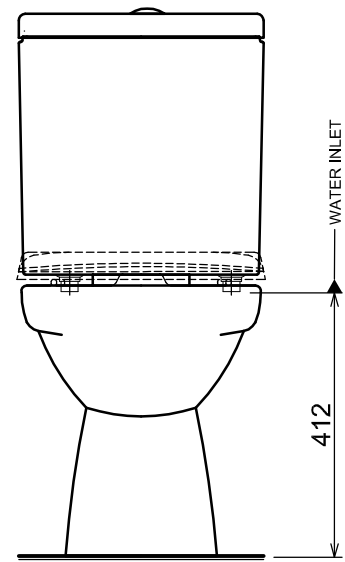
FRONT ELEVATION
