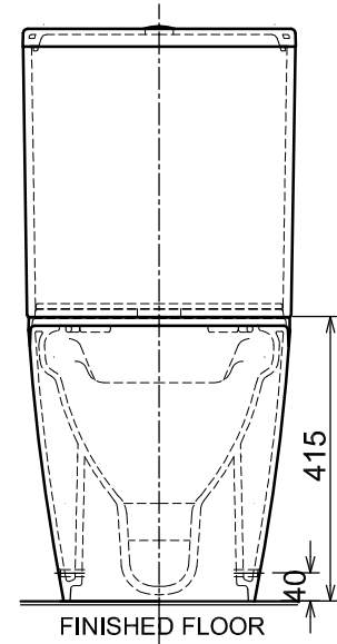
FRONT ELEVATION
