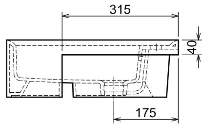
SIDE ELEVATION
