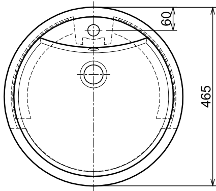
PLAN / TOP ELEVATION
