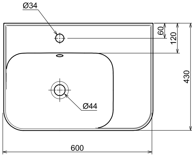
PLAN / TOP ELEVATION
