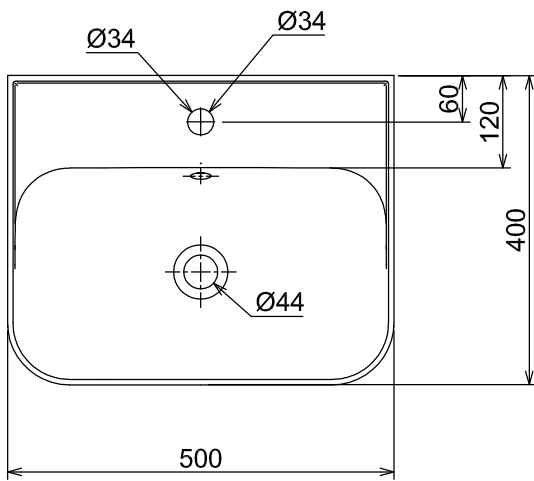
PLAN / TOP ELEVATION
