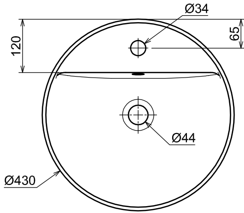
PLAN / TOP ELEVATION
