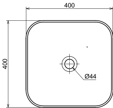
PLAN / TOP ELEVATION
