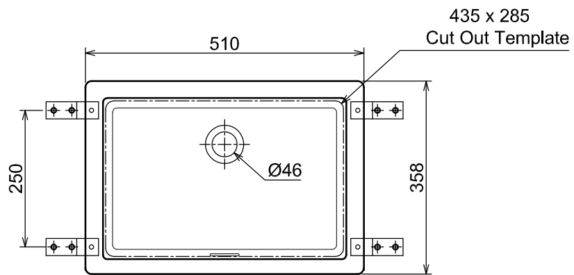
PLAN / TOP ELEVATION
