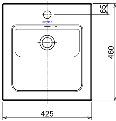
PLAN / TOP ELEVATION
