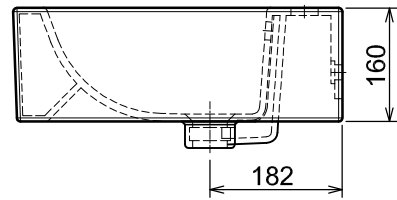
SIDE ELEVATION
