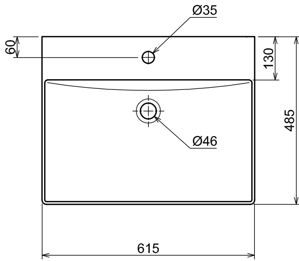
PLAN / TOP ELEVATION
