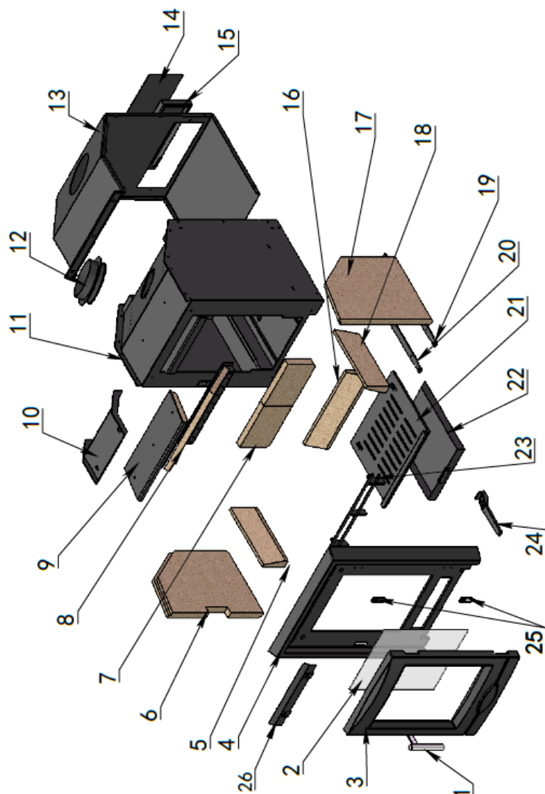
Portland/ Dedham 7kw parts diagram:
