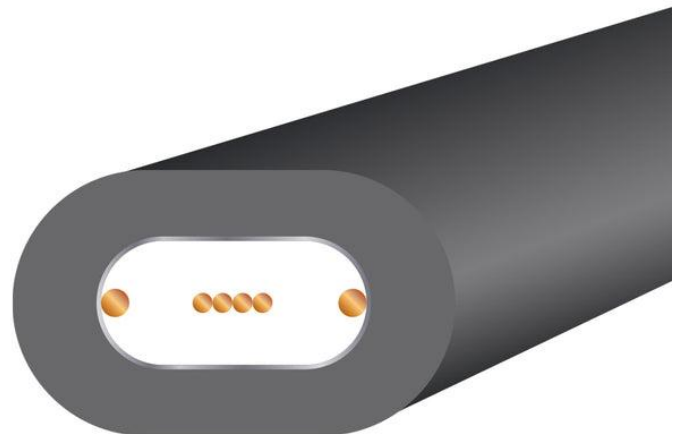
Flexi-Flat™ Design
