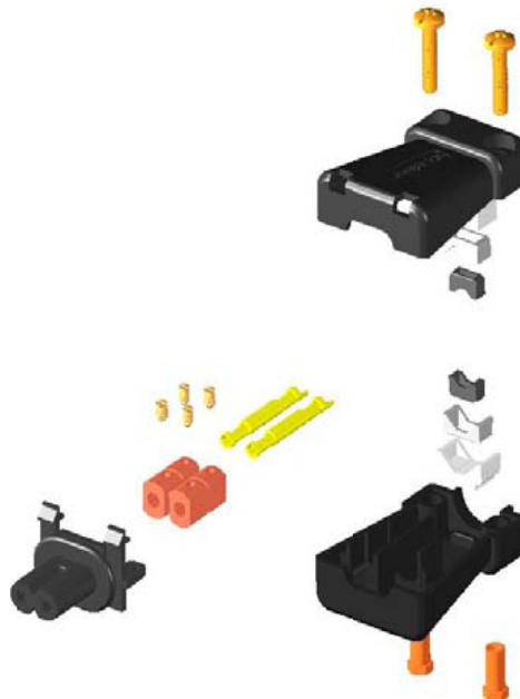
FI-8 N Set screw model construction
