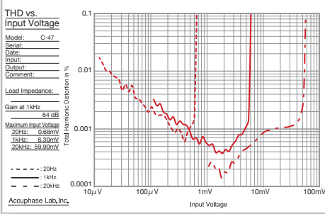
Input voltage vs. THD characteristics (MC input)
