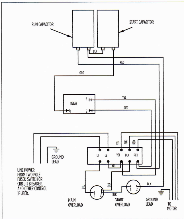
3 hp STANDARD 282 302 8110
