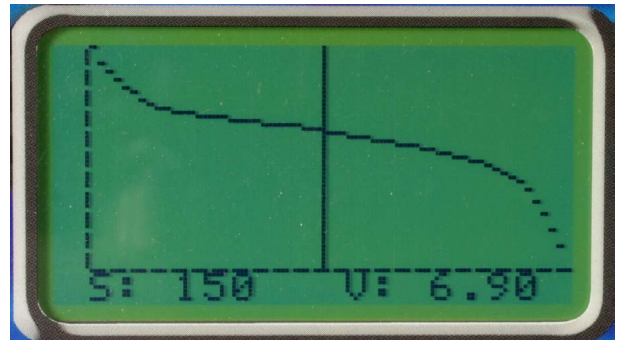
Figure 16: Typical discharge graph
