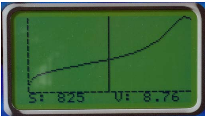
Figure 15: Typical charge graph
