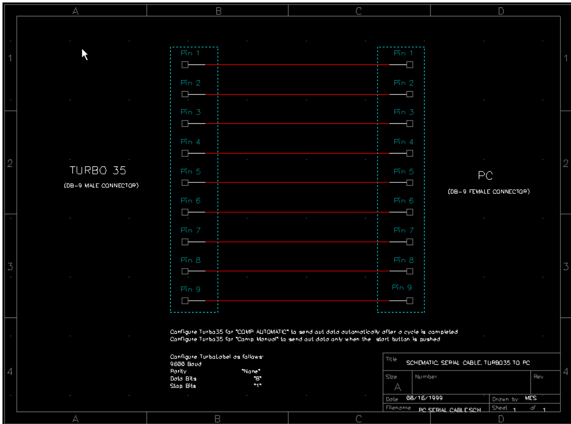
Figure 19: PC Serial Cable for use with T35-GFX
