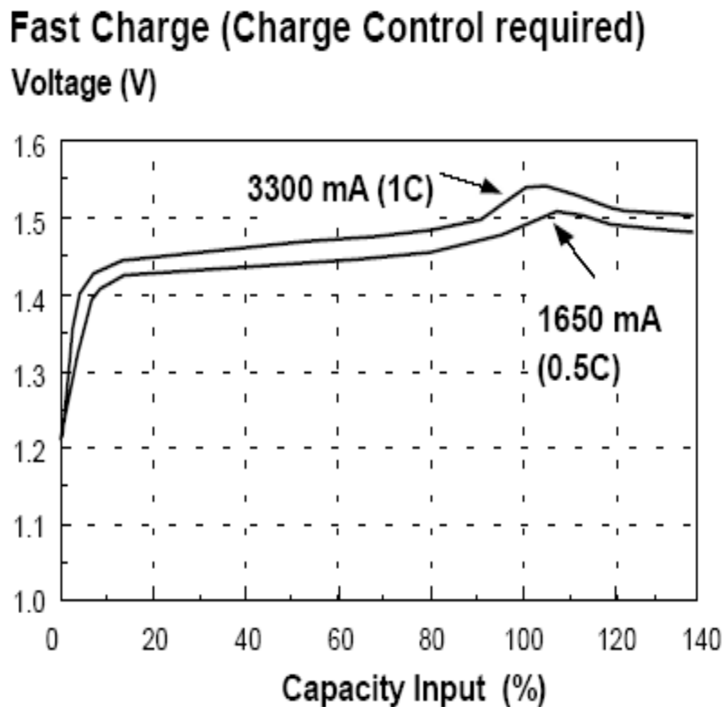
Figure 9: 1C charge profile for 3300 mAhr NimH Cell
