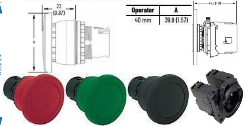
Mushroom Operators (40 mm and 60 mm)
