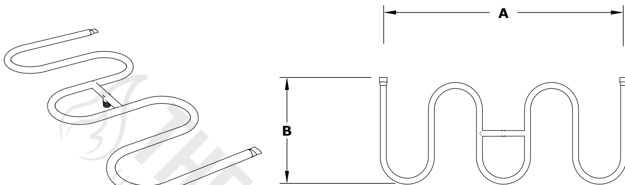
ISOMETRIC VIEW
