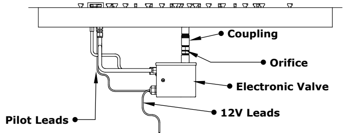
FRONT SIDE VIEW
