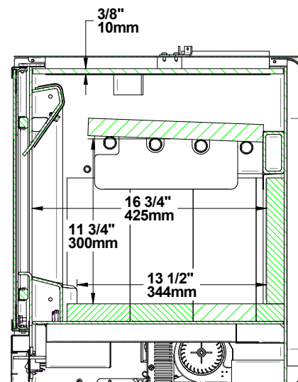
Figure 6: Side Firebox
