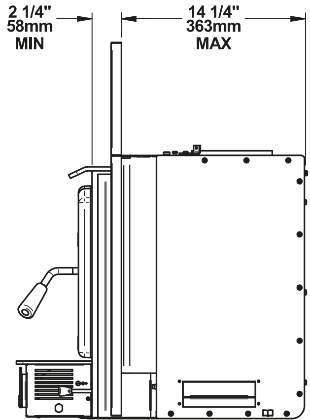
Figure 2 : Side View - Minimum Insert Projection
