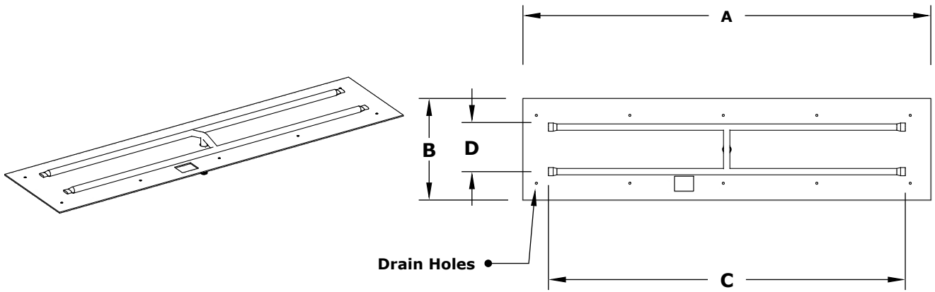
ISOMETRIC VIEW
