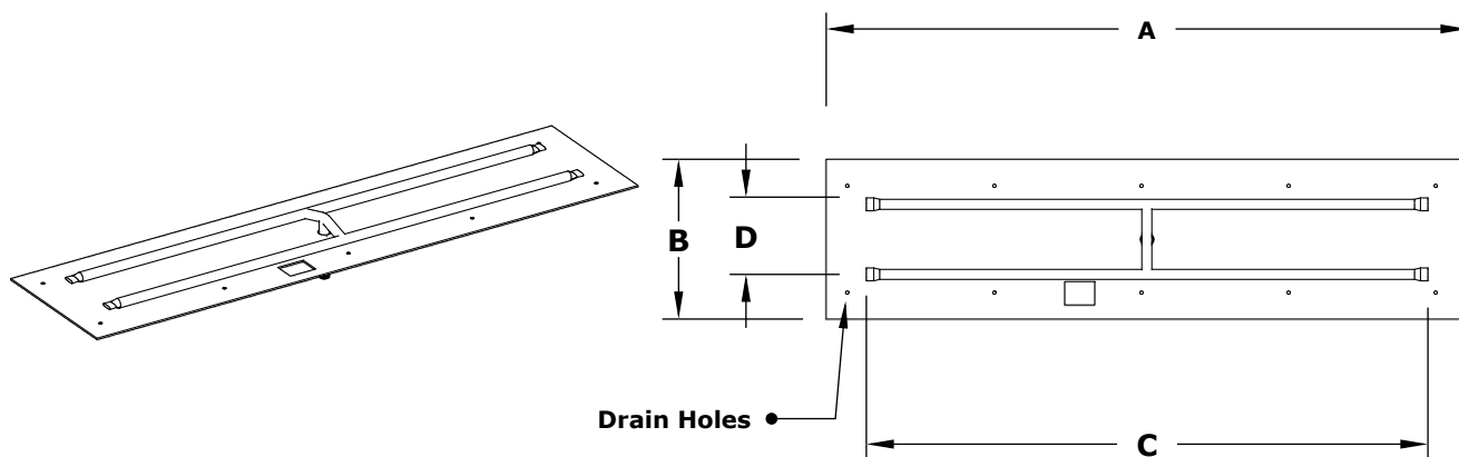
ISOMETRIC VIEW
