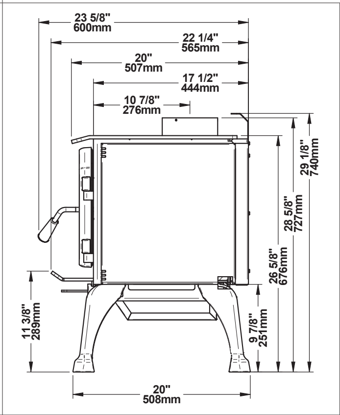
Figure 6: Side View
