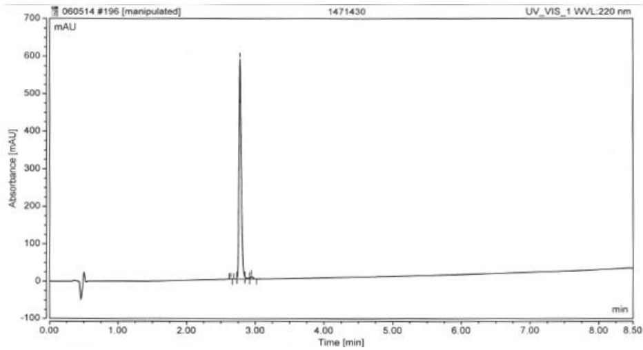
HPLC-RP chromatogram of purified P-109 peptide.
