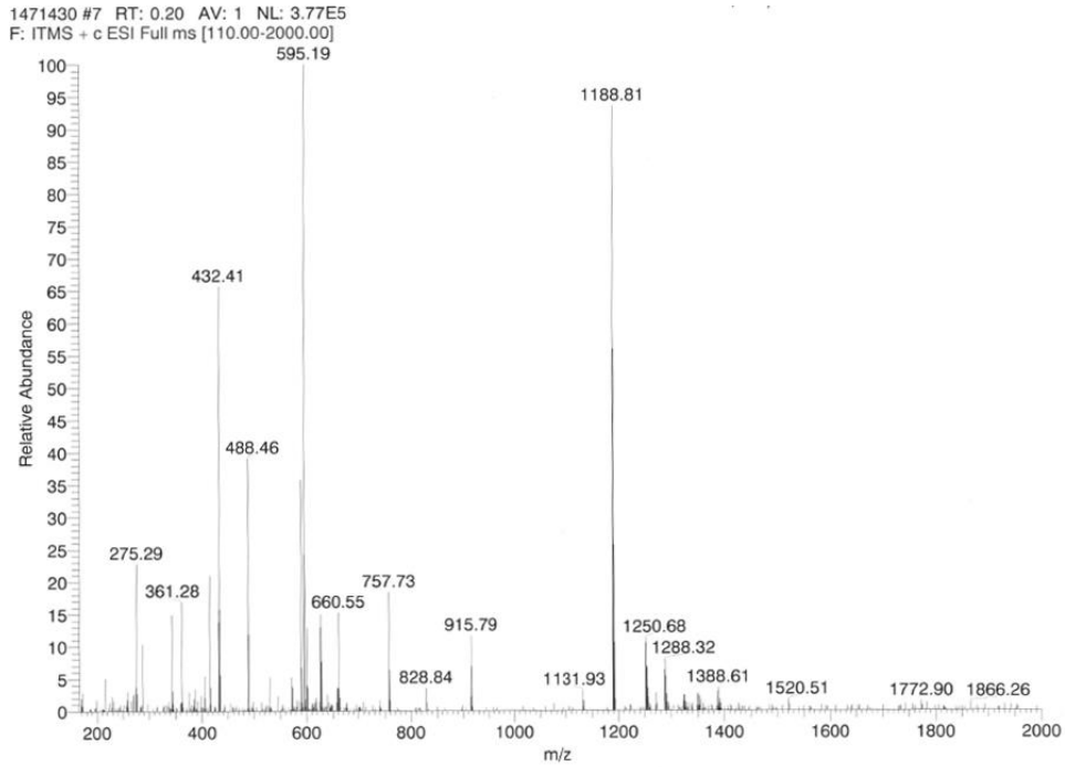
Mass Spec. Data to analyze identity and homogeneity of P-109 peptide.
