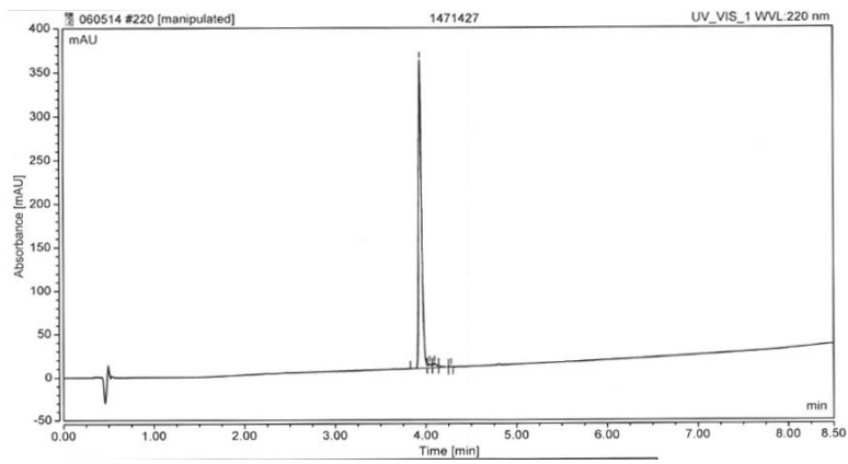
HPLC-RP chromatogram of purified P-106 peptide.
