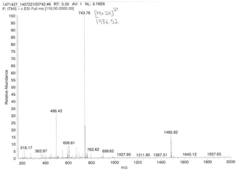
Mass Spec. Data to analyze identity and homogeneity of P-106 peptide.
