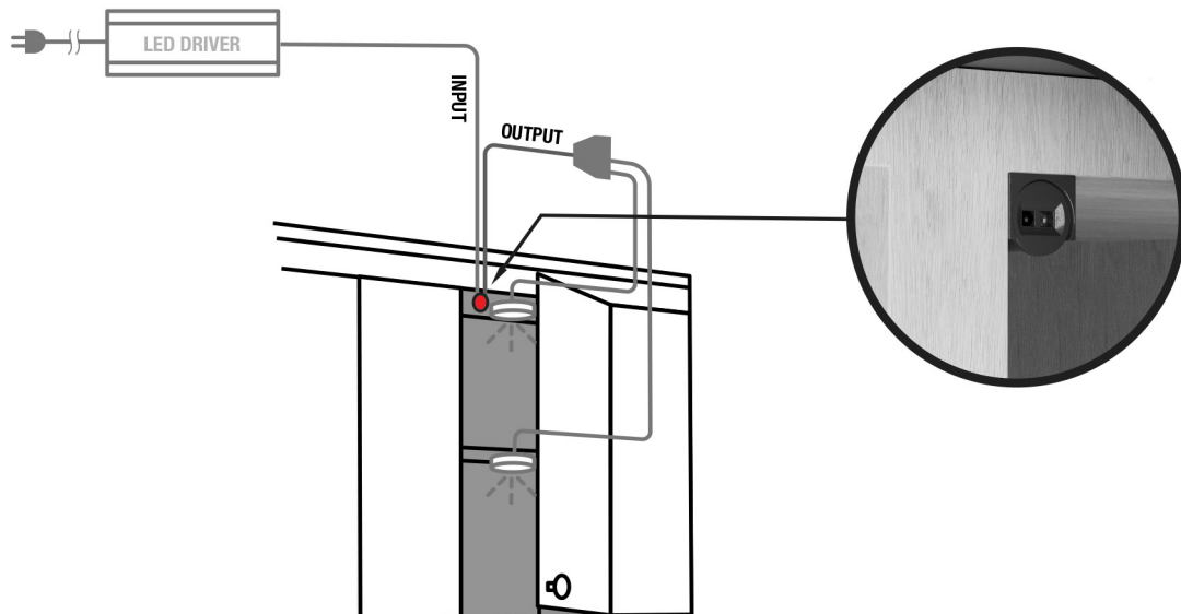
recessed installation drill hole 12mm
