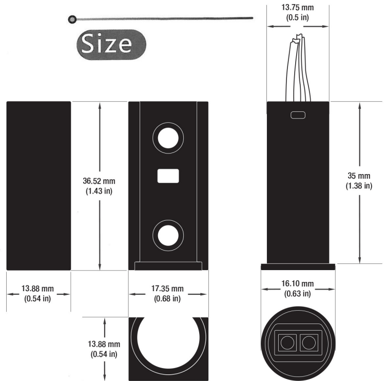
recessed installation drill hole 12mm
