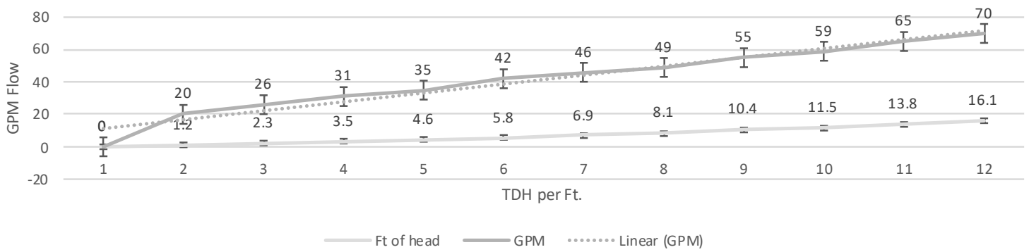
Head Loss
