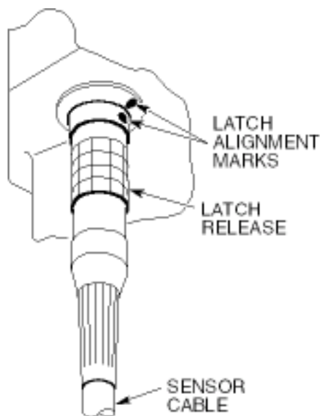
Figure 4. Sensor disconnect
