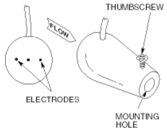
Figure 7. Open-Channel-Velocity Sensor
