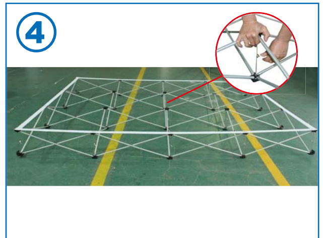
Connect all the steel hooks
