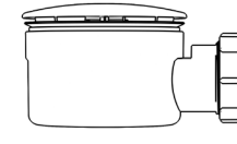
Product Code: WTS40 Description: 1½" Shower Trap (90mm Tray) Seal: 50mm
