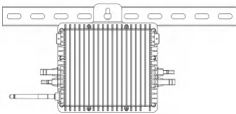
300 / 500G3 (1MPPT) 600 / 800 / 1000G3 (2MPPT) Montage
