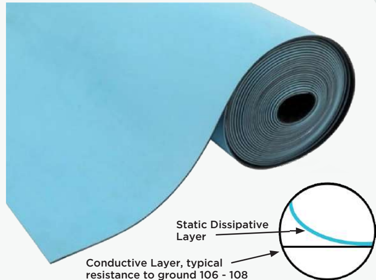
2 Layer Bench Matting Construction
