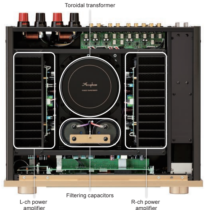
Toroidal transformer
