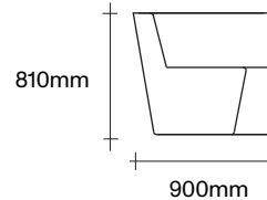
Internal Curved
