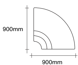
90° External Corner
