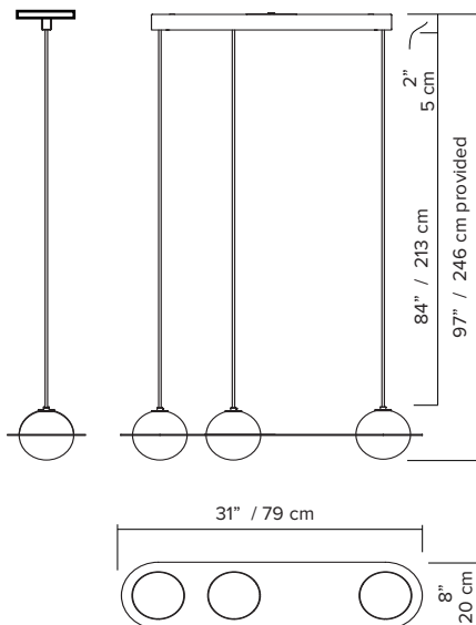
parallel wires
