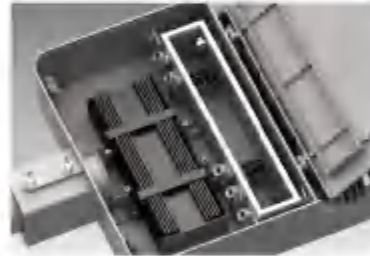
独立的电源腔体和优质硅胶密封。 Independent power supply housing with high quality silicone rubber sealing.
