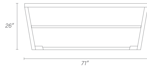
La Roux console table, structure in oak solid wood and base in marble.
