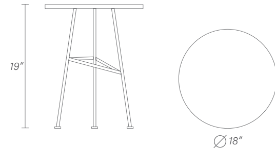
Indie side table, top in marble and structure in iron.
