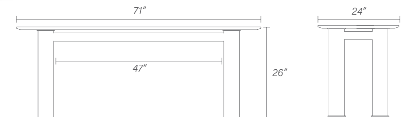
Creta Console, structure in metal or upholstered metal. Top in marble or glass.
