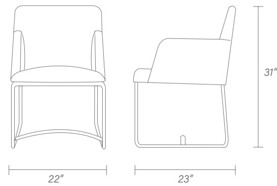
Testino dining chair, upholstered in leather or fabric, base in steel.
