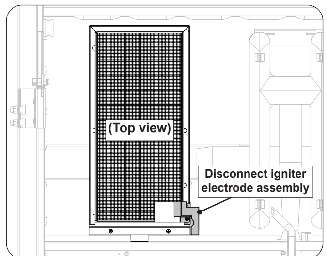
Fig. 46-3 Infrared burner removal
