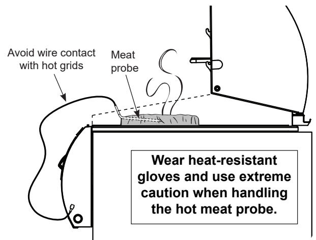
Fig. 34-3 Meat probe
