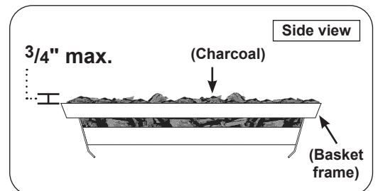
Fig. 41-2 Charcoal loading detail
