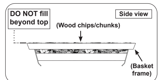
Fig. 41-4 Chips/chunks loading detail
