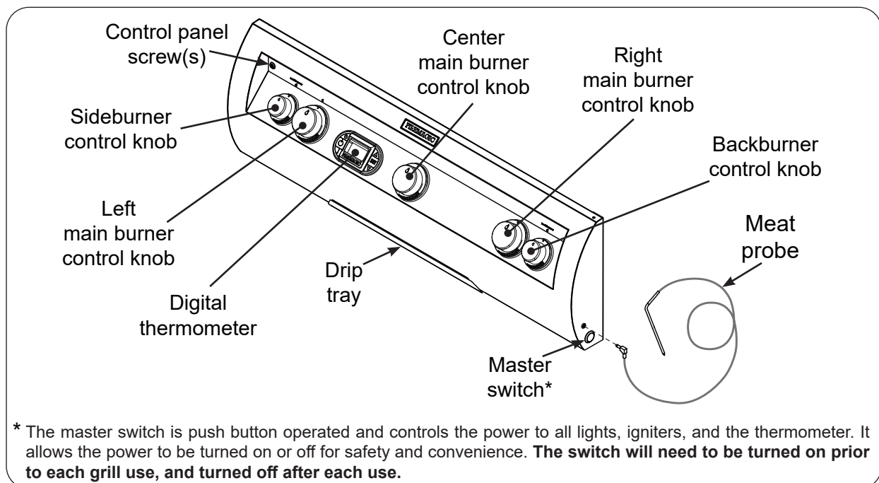
Fig. 29-4 E660s and E790s controls
