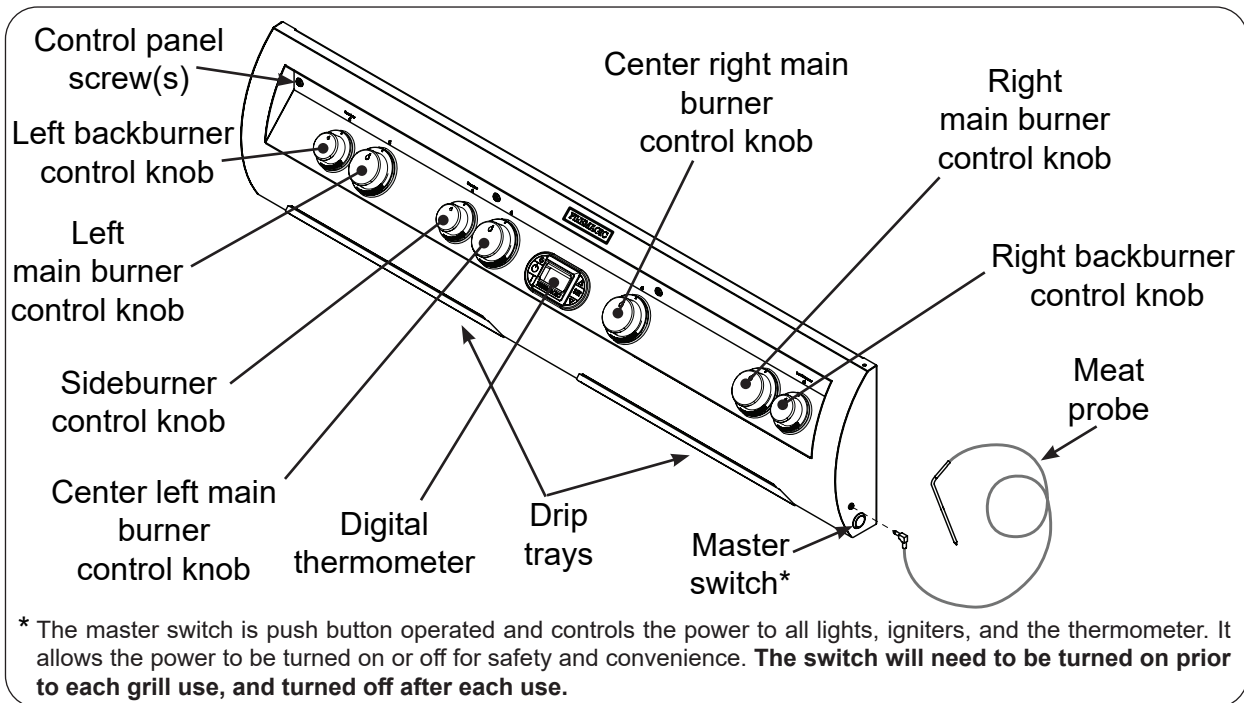
Fig. 29-1 E1060s controls
