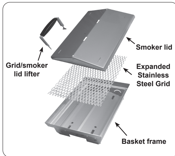
Fig. 40-1 Charcoal/smoker basket items
