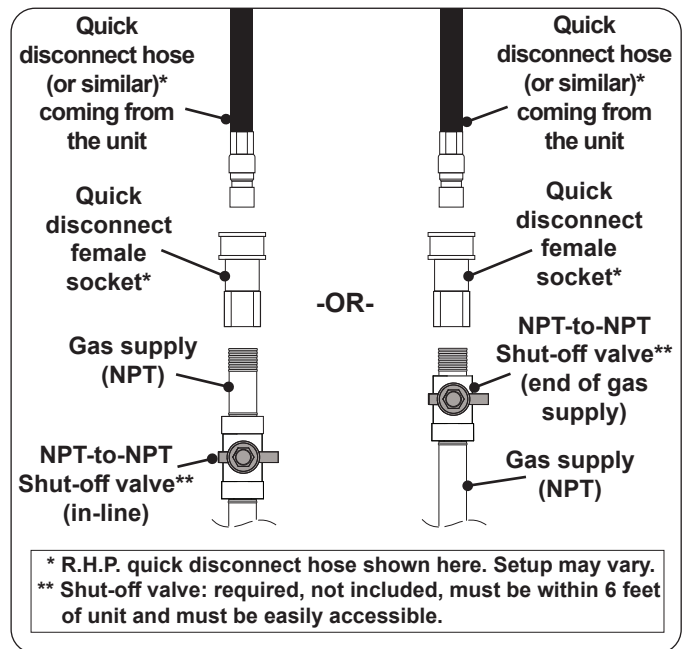
Fig. 24-2 Connecting to a gas line
