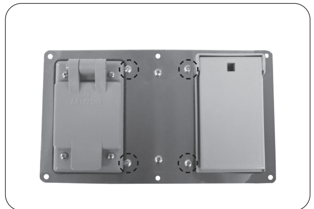
Fig. 48-3 Remove 4 small screws
