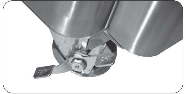
Fig. 23-1 Lock/unlock wheels
