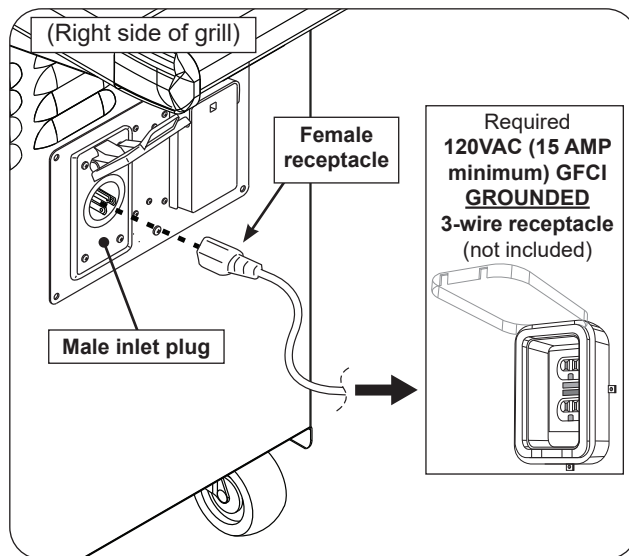
Fig. 28-3 Connect to line power
