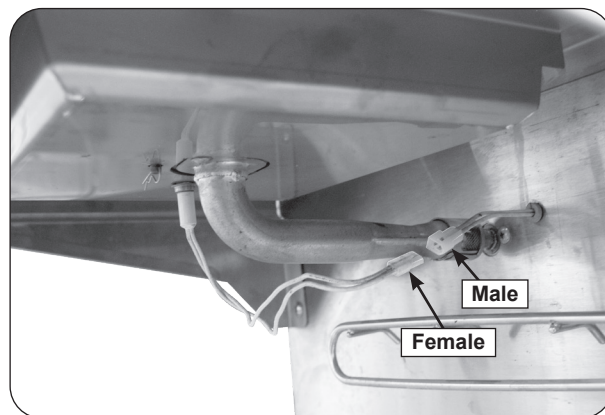
Fig. 28-1 Igniter wire connection
