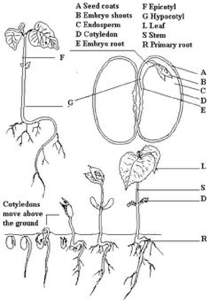
9.3.52 Epigeal germination of bean
