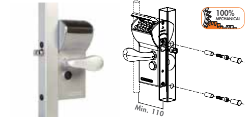
LF – Mechanical Code lock Free Exit
