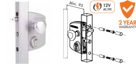
LE – Electric lock
