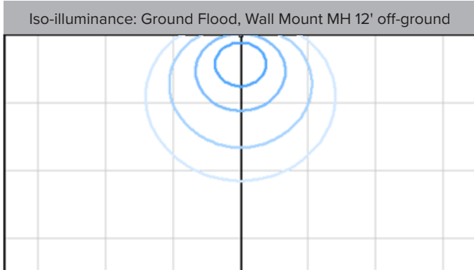
Foot-candles: 0.1, 0.2, 0.5, 1 | Grid spacing 20'
