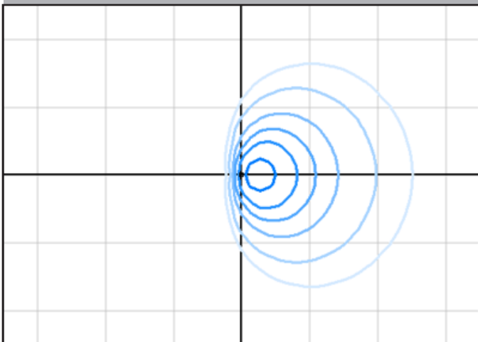
Iso-illuminance: Ground Flood, Wall Mount MH 8' off-ground
