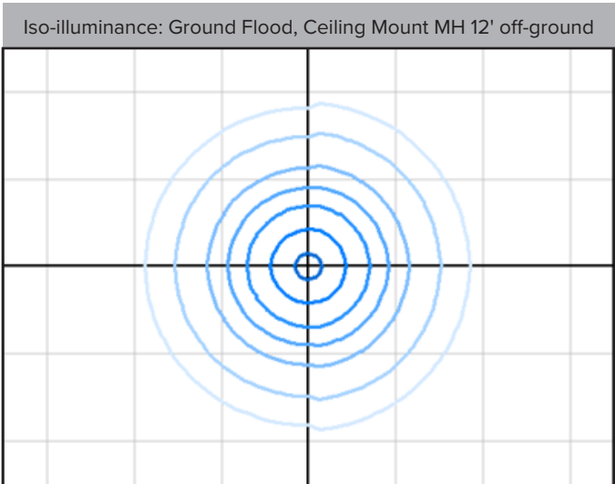
Foot-candles: 0.1, 0.2, 0.5, 1, 2, 5, 10 | Grid spacing 20'
