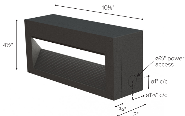
Luminaire Housing with integrated Concrete Pour Box
