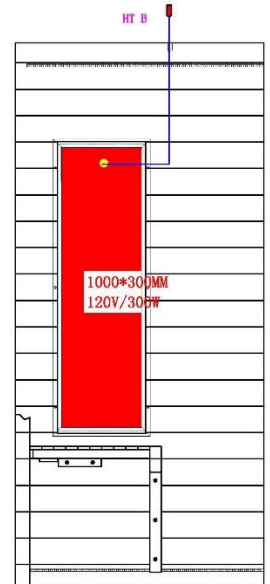
Right side wall panel
